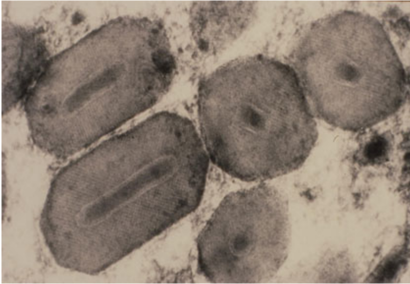
Fig. 2: Until now very effective in pest management: the granulovirus.
